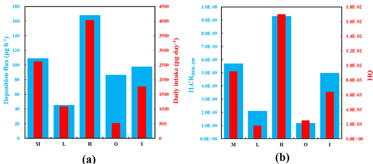
Fig. 6. Deposition fluxes, daily intake, hazard quotient (HQ) and ILCR BDE-209 values of HFRs under different conditions. M is the total mean value, L is light pollution conditions, H is heavy pollution conditions, O is outdoor conditions, and I is indoor conditions.
