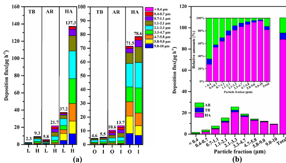
Fig. 5. HFR deposition flux and relative amounts in three human respiratory tracts. HA is the head airway, TB is the tracheobronchial region, AR is the alveolar region, L is light pollution conditions, H is heavy pollution conditions, O is outdoor conditions, and I is indoor conditions.
