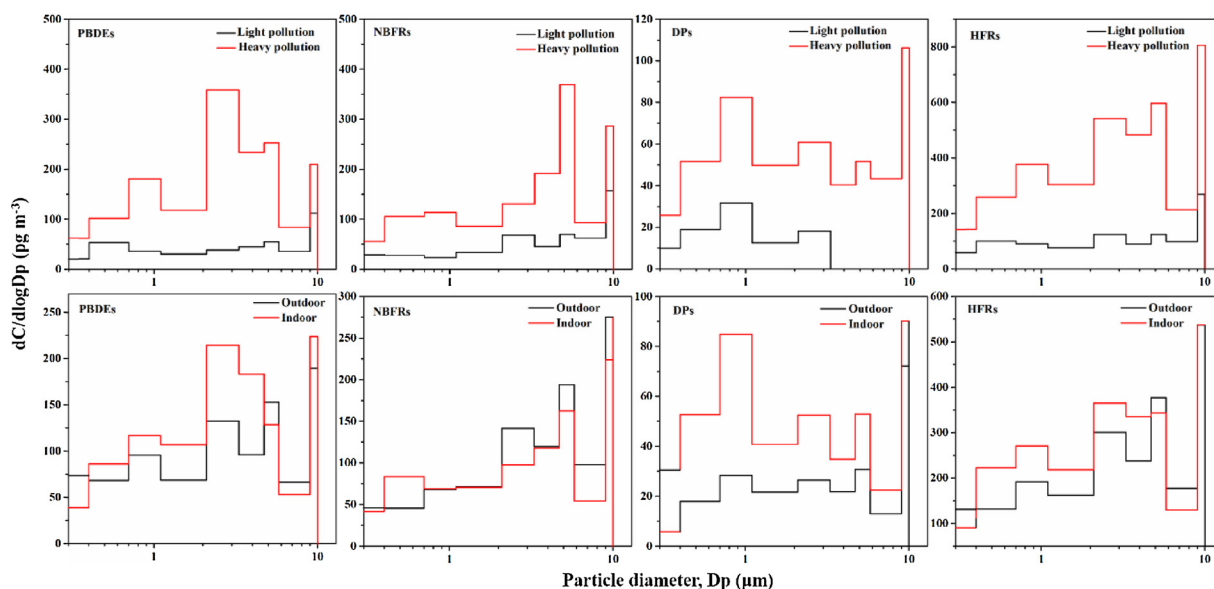
Fig. 4. Mean normalized size distributions of PBDEs, NBFrs and DPs, where dC is the mass concentration on each filter, and dlogDp is the logarithmic aerodynamic diameter ( D_p ) size interval for each impactor stage.
