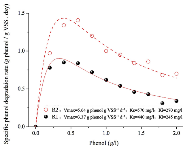
Fig. 2. Batch phenol degradation test with AS from R1 and R2.
