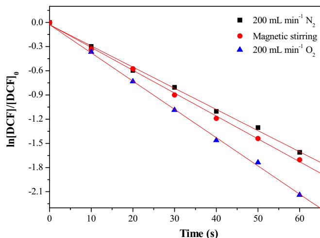
Fig. 4. Kinetics of DCF oxidation by \text{ClO}_2 at various dissolved oxygen contents. [\text{DCF}]_0 = 3.00 \mu\text{M} , [\text{ClO}_2]_0 = 18.9 \mu\text{M} , \text{pH} = 7.0 , 298 \text{ K} .
