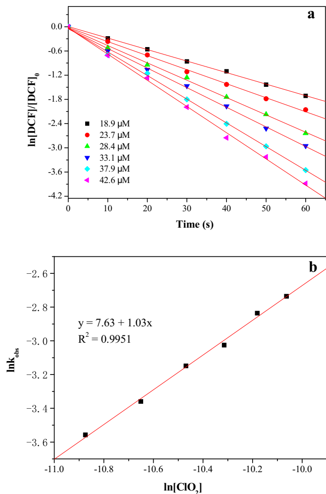
Fig. 1. Determination of reaction order for DCF oxidation by \text{ClO}_2 : (a) plot of \ln([\text{DCF}]/[\text{DCF}]_0) vs. reaction time at different initial \text{ClO}_2 concentrations; and (b) plot of \ln(k_{\text{obs}}) vs. \ln[\text{ClO}_2]_0 . [\text{DCF}]_0 = 3.00 \mu\text{M} , \text{pH} = 7.0 , T = 298 \text{ K} .
