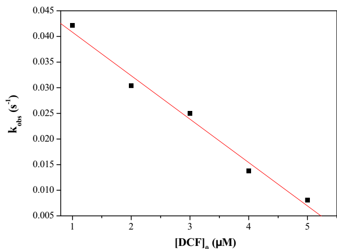
Fig. 6. k_{\text{obs}} for the reactions of DCF with \text{ClO}_2 (18.9 \mu\text{M} ) as a function of initial DCF concentration (1.00–5.00 \mu\text{M} ) at pH 7.0 and 298 K.
