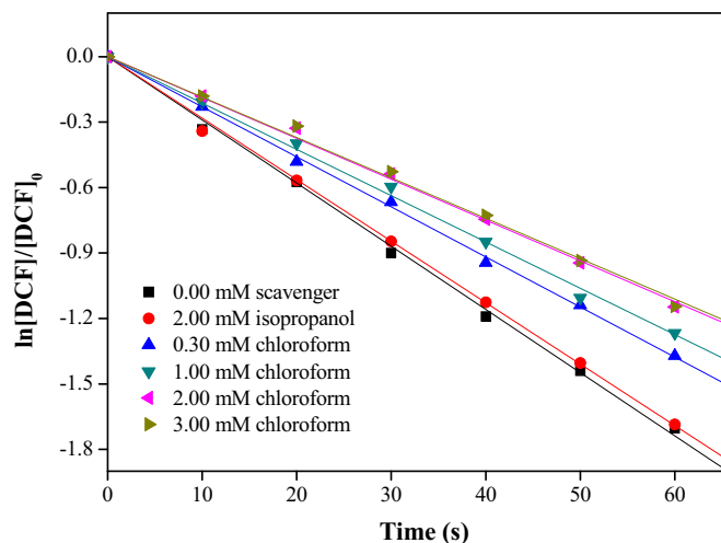
Fig. 5. Effects of isopropanol and chloroform on kinetics of DCF ( 3.00 \mu\text{M} ) oxidation by \text{ClO}_2 ( 18.9 \mu\text{M} ) at \text{pH} 7.0 and 298 \text{ K} .
