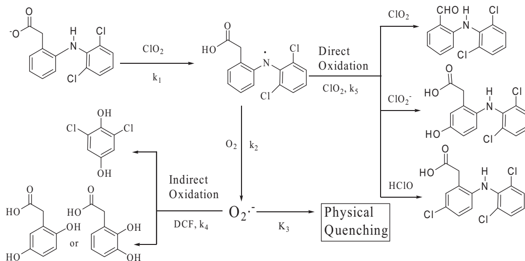
Scheme 1. Proposed mechanism for the initial reactions between DCF and \text{ClO}_2 .
