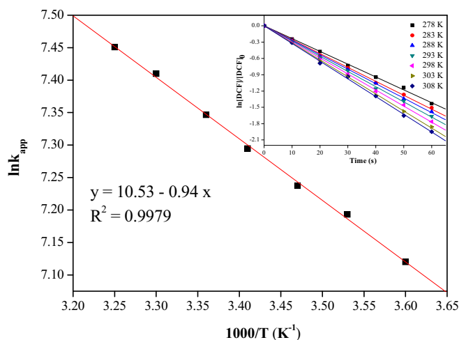
Fig. 3. Arrhenius plot of \ln k_{app} vs. 1/T (insert: plot of \ln[DCF]/[DCF]_0 vs. reaction time under different temperature). [DCF] 0 = 3.00 μM, [ClO 2 ] 0 = 18.9 μM, pH = 7.0.
