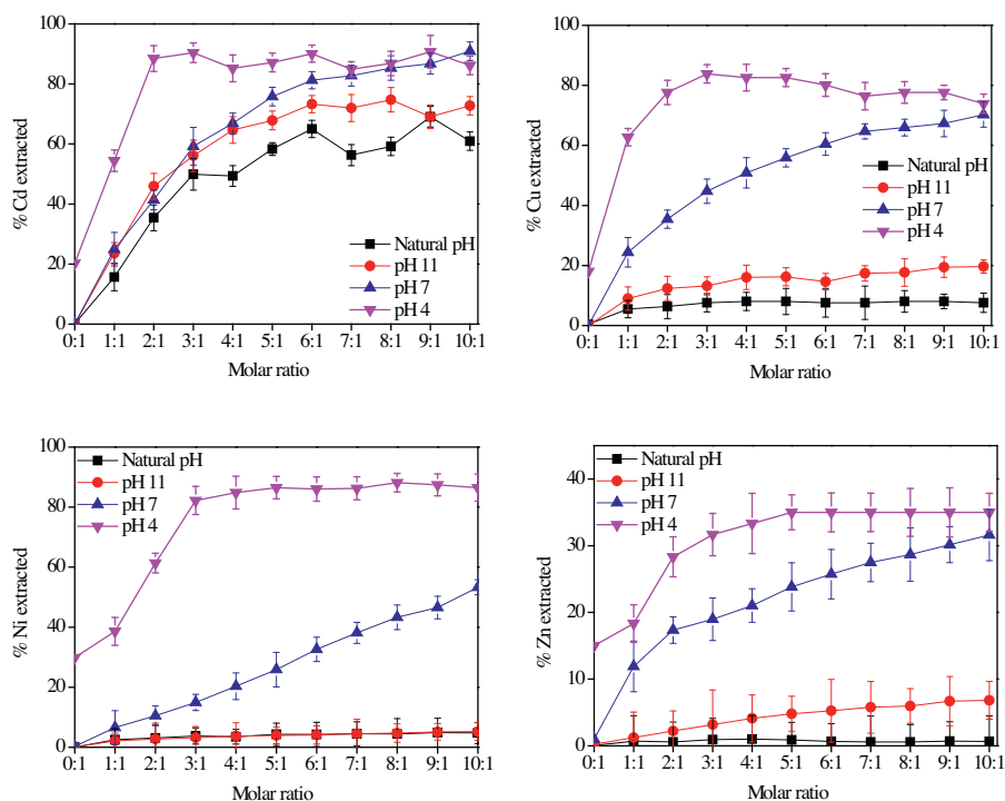
Fig. 4. Effect of the GLDA concentration on the extraction of Cd, Ni, Cu and Zn at natural pH (12–13), pH = 11, pH = 7, and pH = 4.
