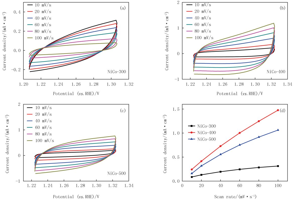
图6 样品NiCo-300(a), NiCo-400(b), NiCo-500(c)在不同扫速下的CV曲线和扫速-电流密度的线性拟合曲线(d) Fig.6 CV curves of NiCo-300(a), NiCo-400(b), NiCo-500(c) at different scan rates and linear fitting curves of current density at different scan rates(d)
