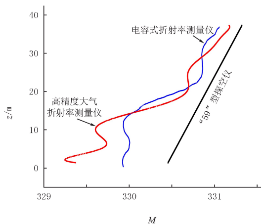
图8 垂直梯度修正折射率测量对比 Fig.8 Comparison of different testing vertical gradient correction for refractive index
