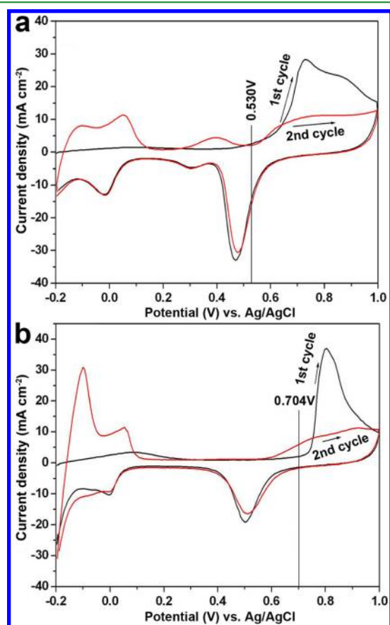
Figure 3. CO-stripping voltammograms of (a) the PdCu/MWCNTs and (b) the Pd/MWCNTs.
