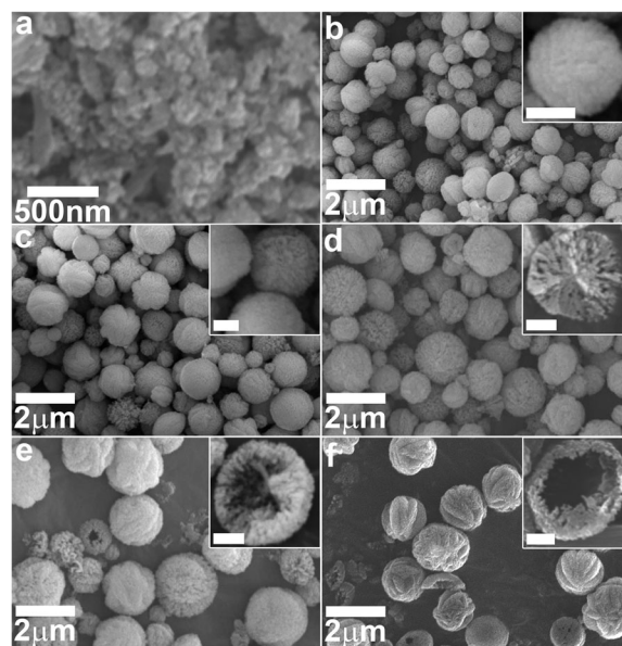
Fig. 2 SEM images showing the evolution of CaCO 3 /FA HSs after different reaction times: (a) 0.5; (b) 3; (c) 6; (d) 12; (e) 18; and (f) 24 h. Insets: Magnified SEM images; scale bars 500 nm.
